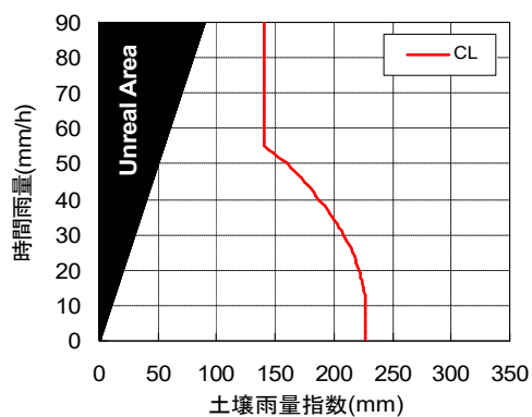
36330604 (RBFN出力値0.2)
