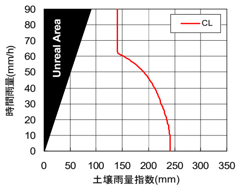
35320814 (RBFN出力値0.2)
